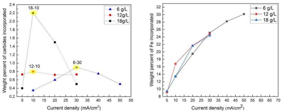
Fig. 6. The effect of current density on the weight percentage of a) TiC and SiC carbides, and b) Fe incorporated in the Ni-Fe (Si-Ti) C composite coating
