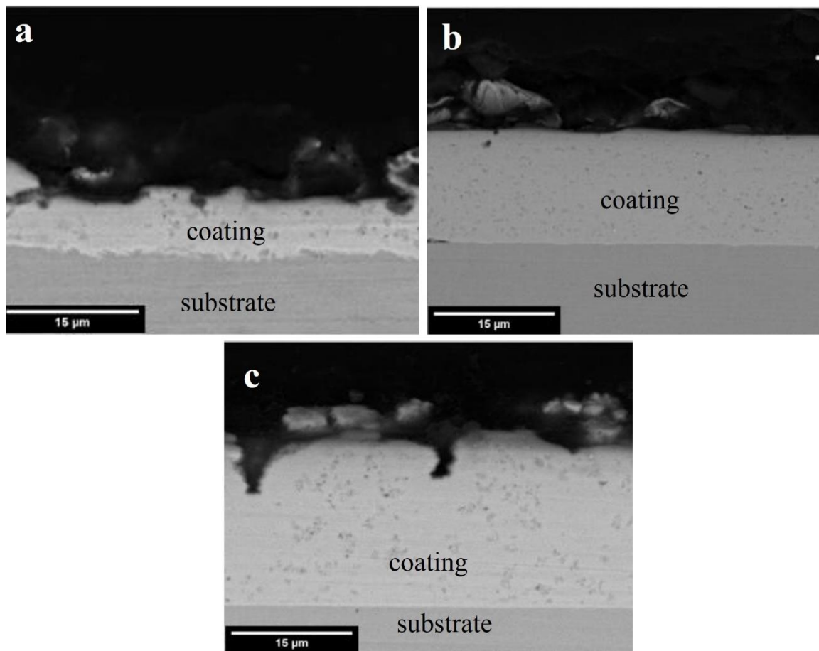
Fig. 3. Cross-sectional SEM micrographs of Ni-Fe (Si-Ti)C composite coatings: a) 6-30, b) 12-10, c) 18-10
